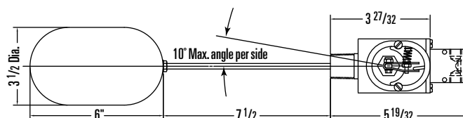
1" NPT THREAD WITH STD. FLOAT AND ARM
