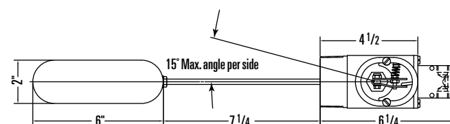
2" NPT THREAD WITH STD. FLOAT AND ARM
